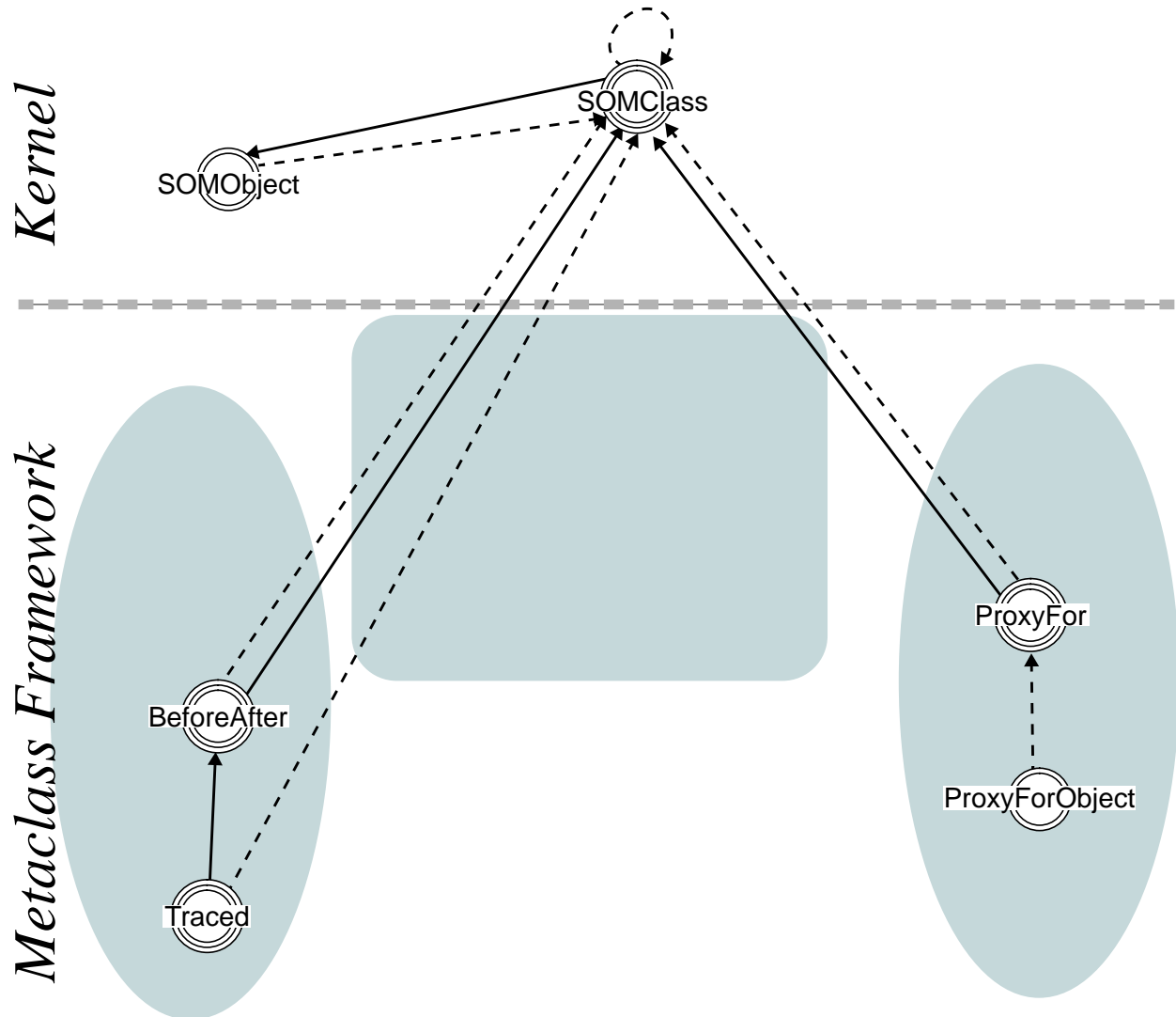
Figure 11. The public view of the Metaclass Framework.
