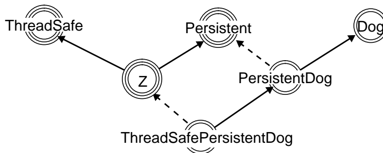
Figure 3. Z must be the class that is both ThreadSafe and Persistent .
