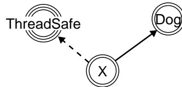
Figure 12. Modifying a class with a Metaclass.
