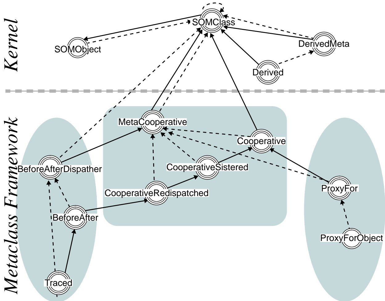
Figure 9. The additional part of the Metaclass Framework for before/after and proxies.
