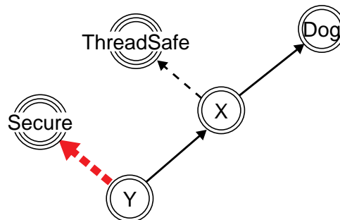
Figure 13. Implicitly Composed Metaclasses.
