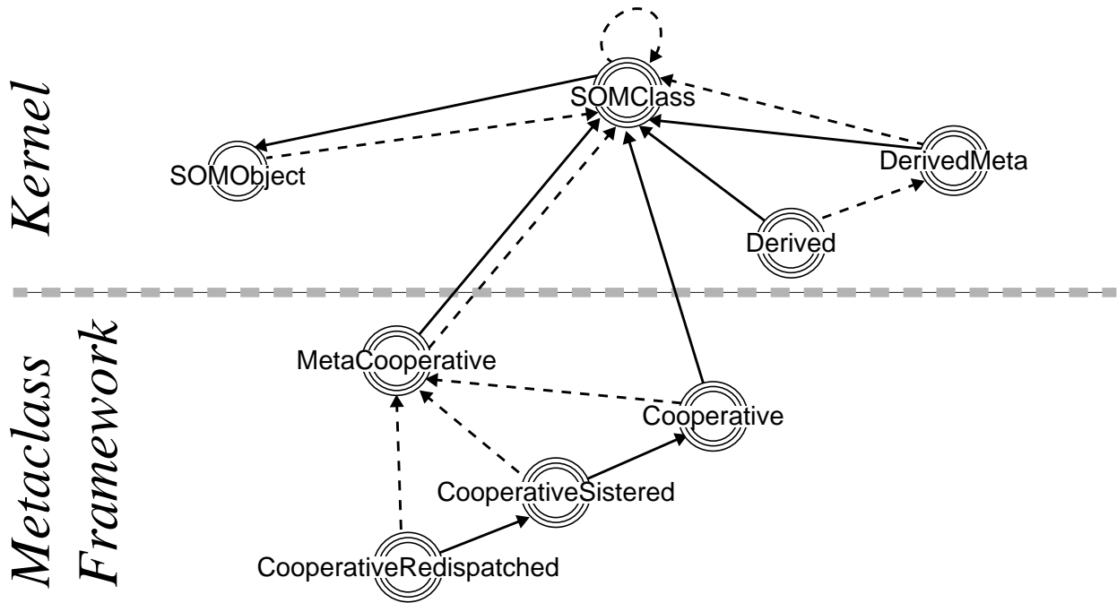
Figure 8. The metaclasses of the subframework for metaobject cooperation.
