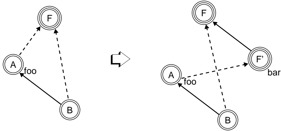
Figure 6. Evolution of a class.
