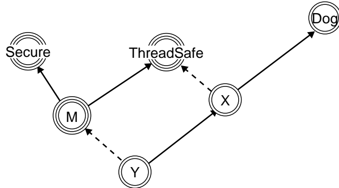
Figure 14. Explicit Composition of Metaclasses.
