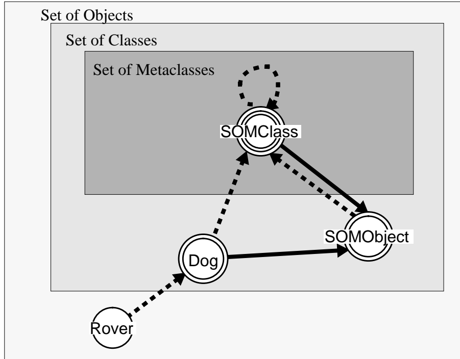
Figure 2. Example of various SOM objects.
