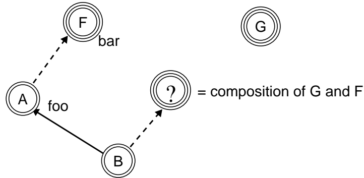
Figure 5. Programmer needs to include property implemented by G.
