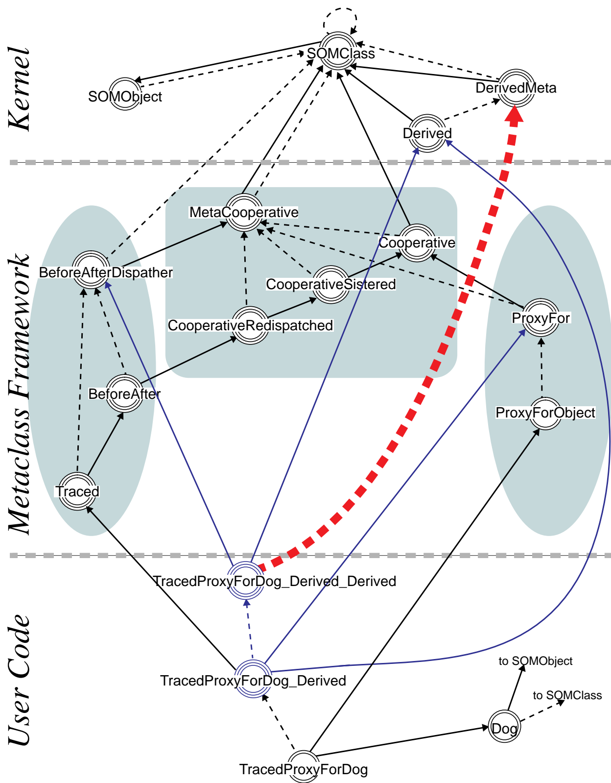
Figure 10. The complexity of creating a traced proxy for Dog.
