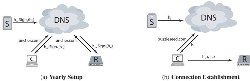
Figure 2: Puzzle Distribution Via DNS. (a) Once a year, a trusted seed generator ( S ) publishes the anchor value h_n of a hash chain, along with a signature on h_n , as a DNS record. By performing a DNS lookup on a well-known name, clients and routers can obtain this record. (b) To establish a capability, the client performs another DNS request. The resulting DNS record contains the current puzzle seed, h_i . The client creates a puzzle based on h_i and includes the puzzle solution ( x ) in its setup packet. The router first verifies the puzzle seed h_i by repeatedly hashing it to get h_n . In most cases, the router will have already seen h_i and hashing will be unnecessary. Finally, the router uses Equation 1 to verify the puzzle solution.
