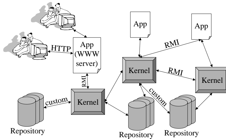
Figure 1. Placeless Documents. Kernels communicate with each other, and with Placeless applications, via RMI. Some applications may be used by multiple users at the same time. Kernels might need to manage documents owned by different users.
