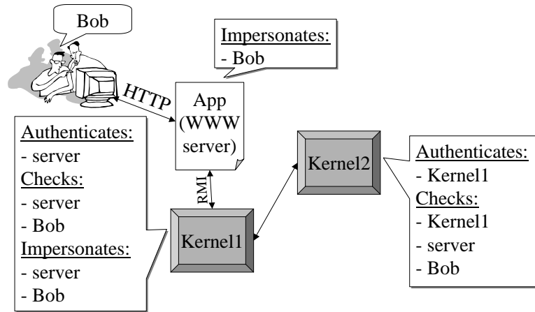
Figure 2. Impersonation in Placeless is similar to a quoting chain in ABLP logic.
