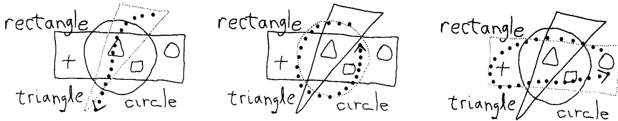
Figure 5: a. A pose model capturing the location and rough shape of emergent objects is equivalent to fitting an oriented bounding box around the object. The triangle and the selection gesture path (depicted with circular dots) share the same pose parameters. b. Nonlinear pose similarity measure (actually a dissimilarity measure whose minimum value of 0 occurs for identical poses). Dissimilarity is expressed as a soft OR function over differences in location, aspect ratio, orientation, and scale. Satisfactory values for the free parameters are \rho_1 = .75 and \rho_2 = .4 . c. Examples of selection by pose matching. Selection gesture paths are depicted in circular dots, resulting selected objects are shown with dotted lines.
