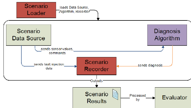
Fig. 1. Run-time architecture
