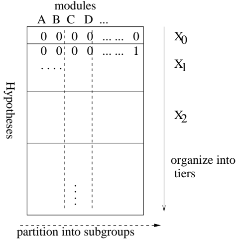
Figure 1: Basic idea: (1) organize hypothesis into tiers (along the vertical direction), and (2) partition components into subgroups (along the horizontal direction), for instance, AB are a group, and CD are a group.
