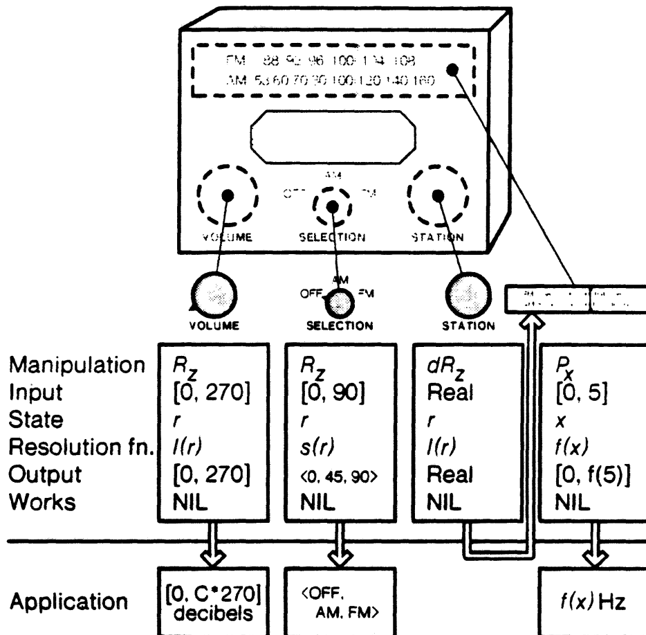
Figure 2. An analysis of a simple radio that illustrates various input devices. Two rotational devices are connected directly to the application. The third rotational device is connected to a positional device, which is then connected to the application.
