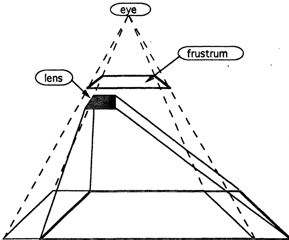
Figure 4: (a) Illustration of how the truncated pyramid may leave the viewing frustum if lens movement is not coupled to viewpoint movement. (b) The frustum after viewpoint movement.
