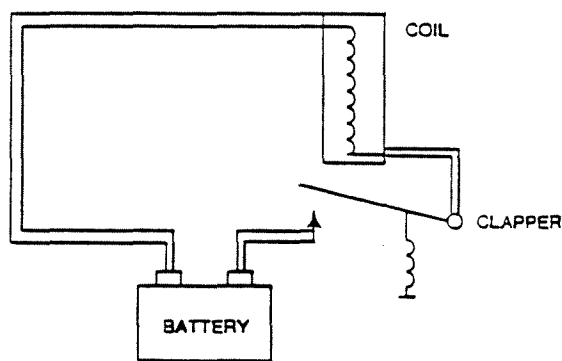
Figure 1 : Buzzer
