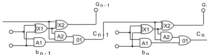
Figure 1: An n -bit ripple carry adder.
