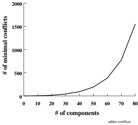
Figure 4: Number of minimal conflicts vs. number of gates.
