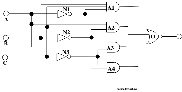
Figure 2: A 3-bit parity circuit is cascaded to obtain an n bit parity circuit.
