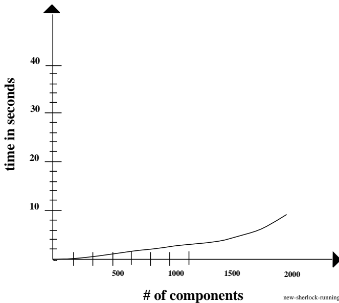
Figure 5: Running time in seconds vs. size in gates (of an adder) on an XL1200
